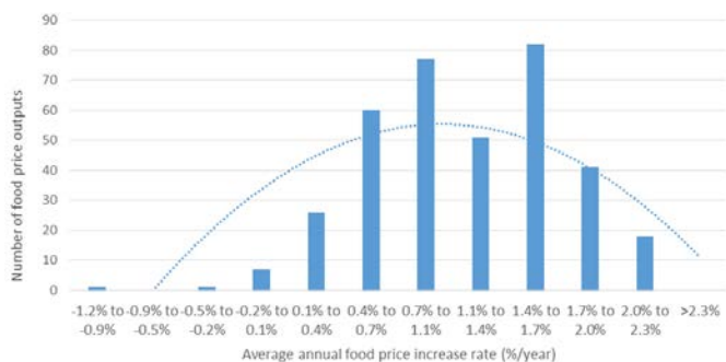
Figure 8-3: Histogram synthesizing the distribution of average annual food price increase rates for all climate change scenarios, 2010-2050
